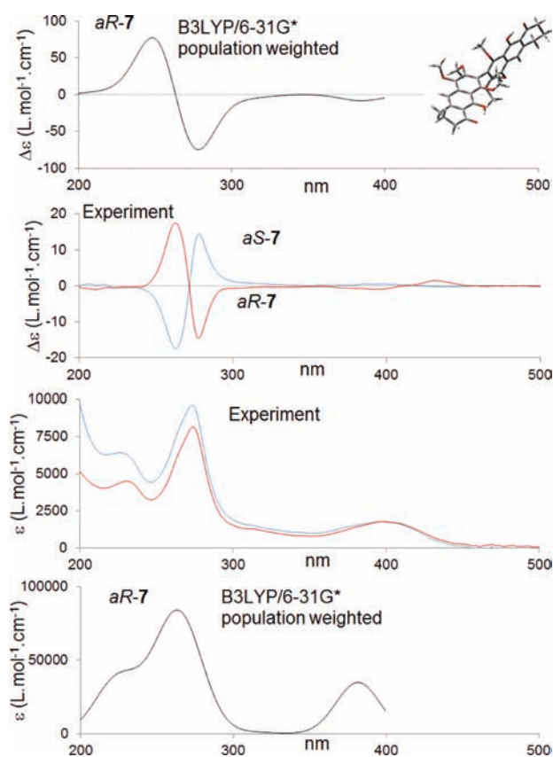
Figure 3. ECD and absorption spectra of 7 . Top panel: quantum chemical prediction of ECD spectrum for aR-7 at the B3LYP/6-31G* level; Middle two panels: experimental ECD and absorption spectra of aS-7 (blue) and aR-7 (red); Bottom panel: quantum chemical prediction of absorption spectrum for aR-7 . The inset in the top panel shows the structure of lowest energy conformation of aR-7 at the B3LYP/6-31G* level.
